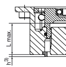
Detail X
