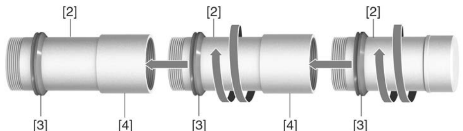
Figure 20: Protection tube made of segments with threaded sleeves
