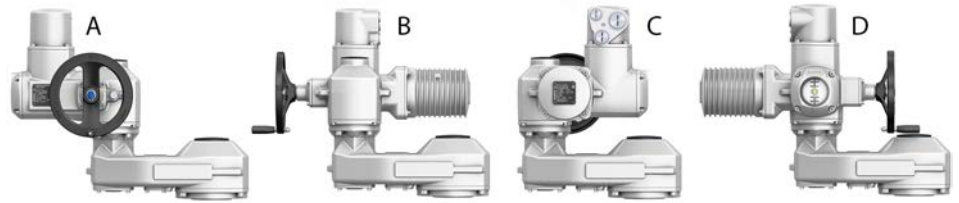
Figure 11: Mounting positions A – D
