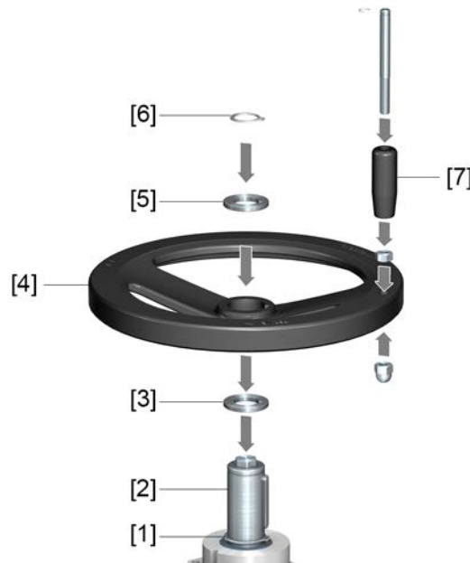
Figure 10: Handwheel
