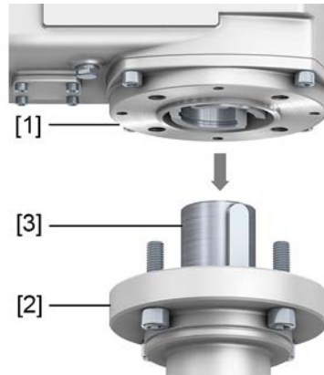
Figure 18: Mounting output drive types B
