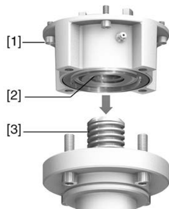
Figure 13: Output drive type A (example of A 10.2)
