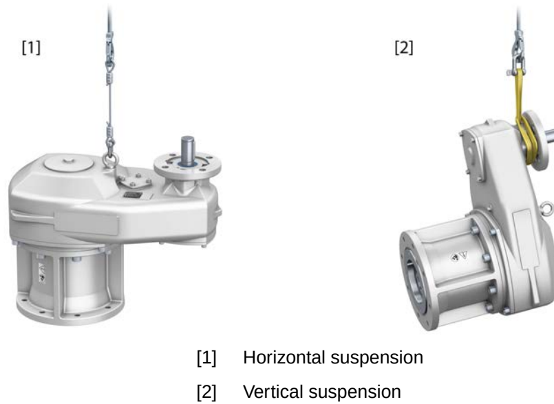
Figure 8: Example of GST 30.1 with horizontal and vertical suspension
