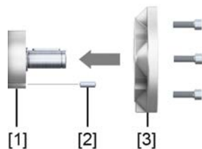
Figure 12: Mount flange to multi-turn gearbox
