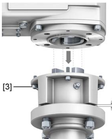
Figure 15: Example of output drive A 10.2
