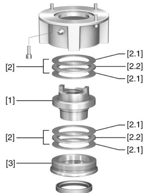
Figure 16: Example of output drive A 10.2
