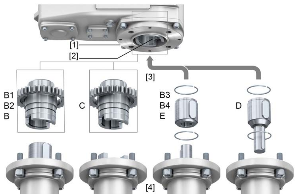
Figure 17: Mounting principle
